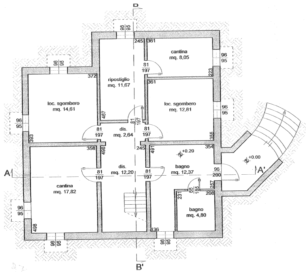
Piano interrato
